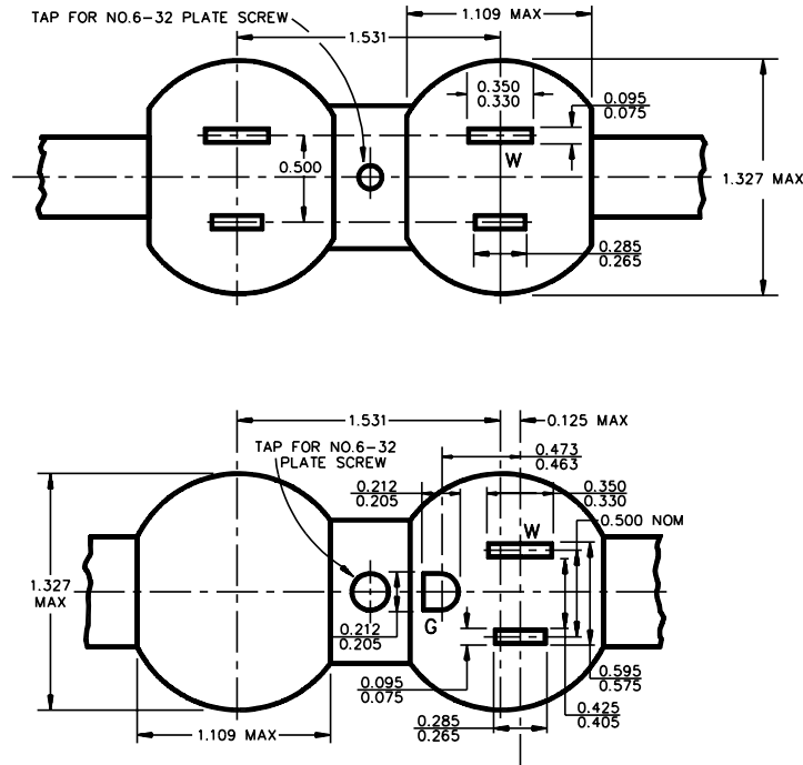
Figure 7.2 125V, 15A Duplex receptacle
