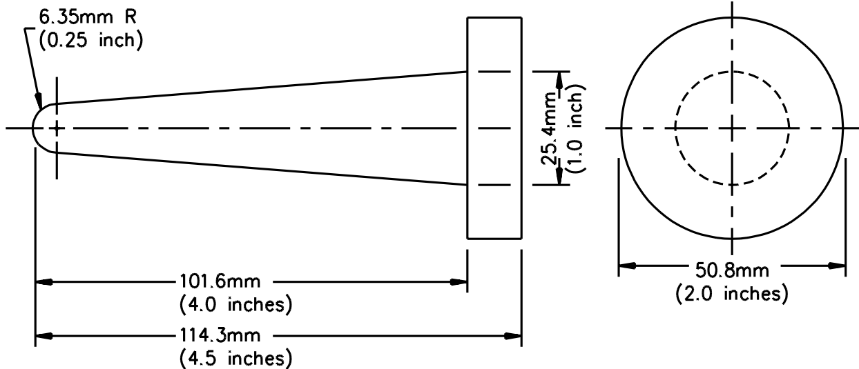
Figure 16.4 Accessibility probe
