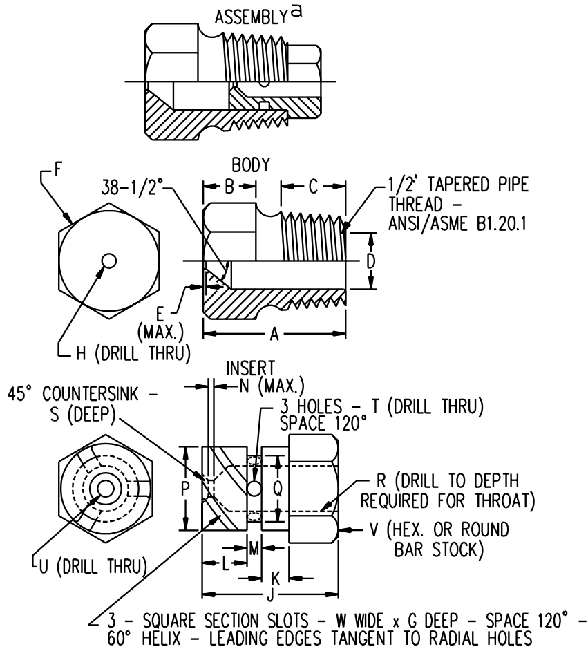
Figure 64.2 Water-spray piping
