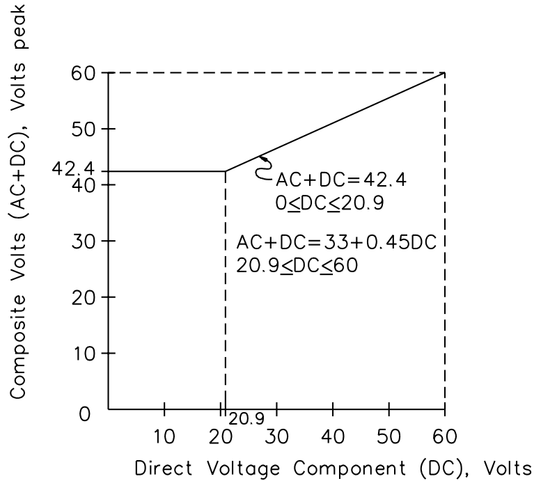
Figure 16.3 Maximum acceptable voltage
