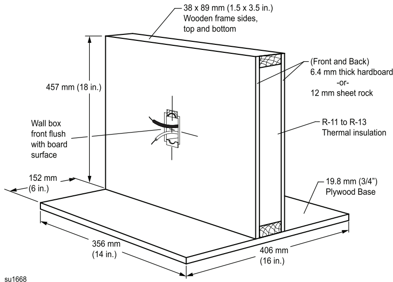
Figure 86.1 Test setup
